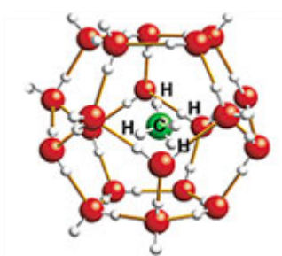
View of a methane hydrates compound
