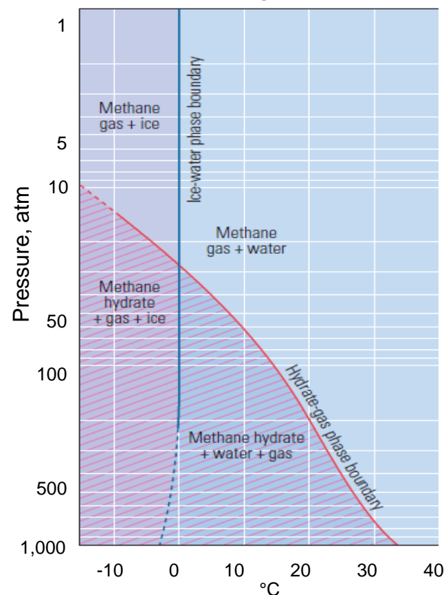
View of a methane hydrates compound
