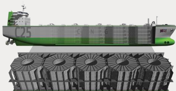
View of Sea NG Coselle™ CNG ship and containment
